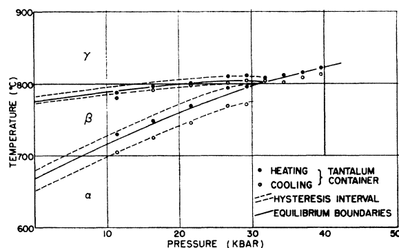
FIG. 3. Phase diagram for uranium obtained by heating and cooling at 3-5°C/sec, sample encapsulated in tantalum. Values for increasing pressure only, but corrected for friction. Proposed hystereses (dotted lines) for 3-5°C/sec rate and true equilibrium boundaries (solid line) for pure uranium.
